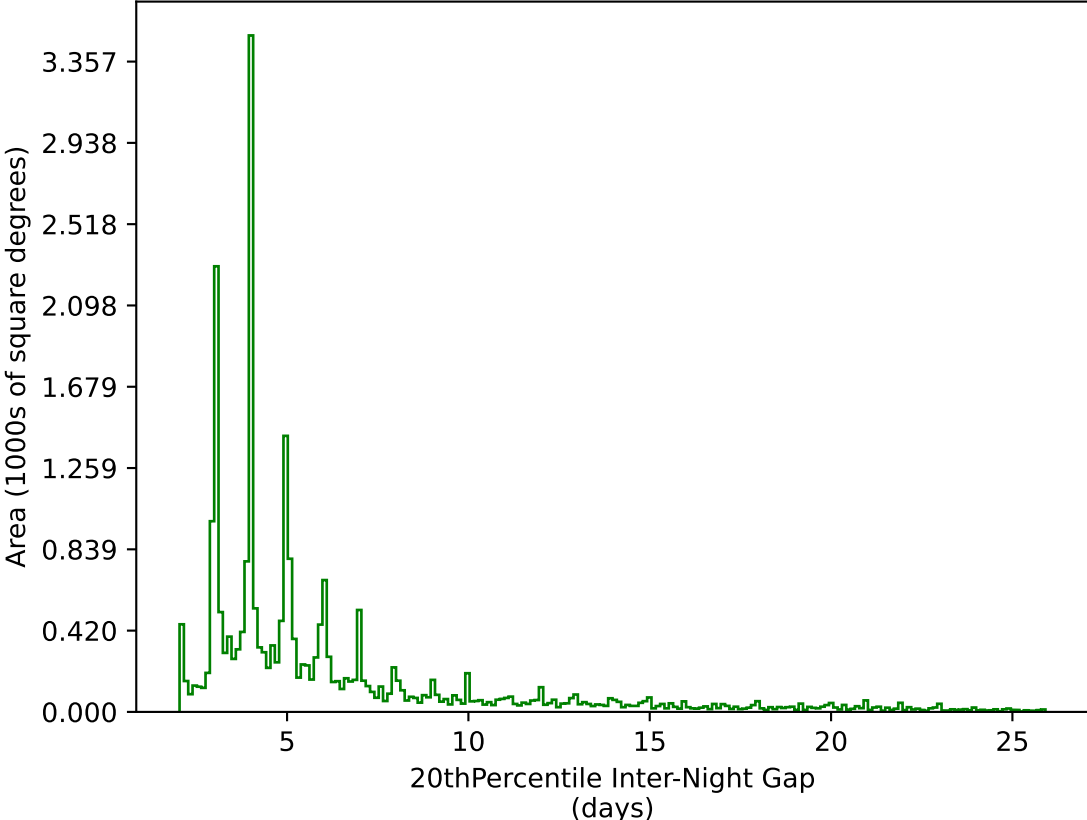
too_elab_2yr_r128_d3_ugrizy_v3.4_10yrs All sky g band: 20thPercentile Inter-Night Gap
