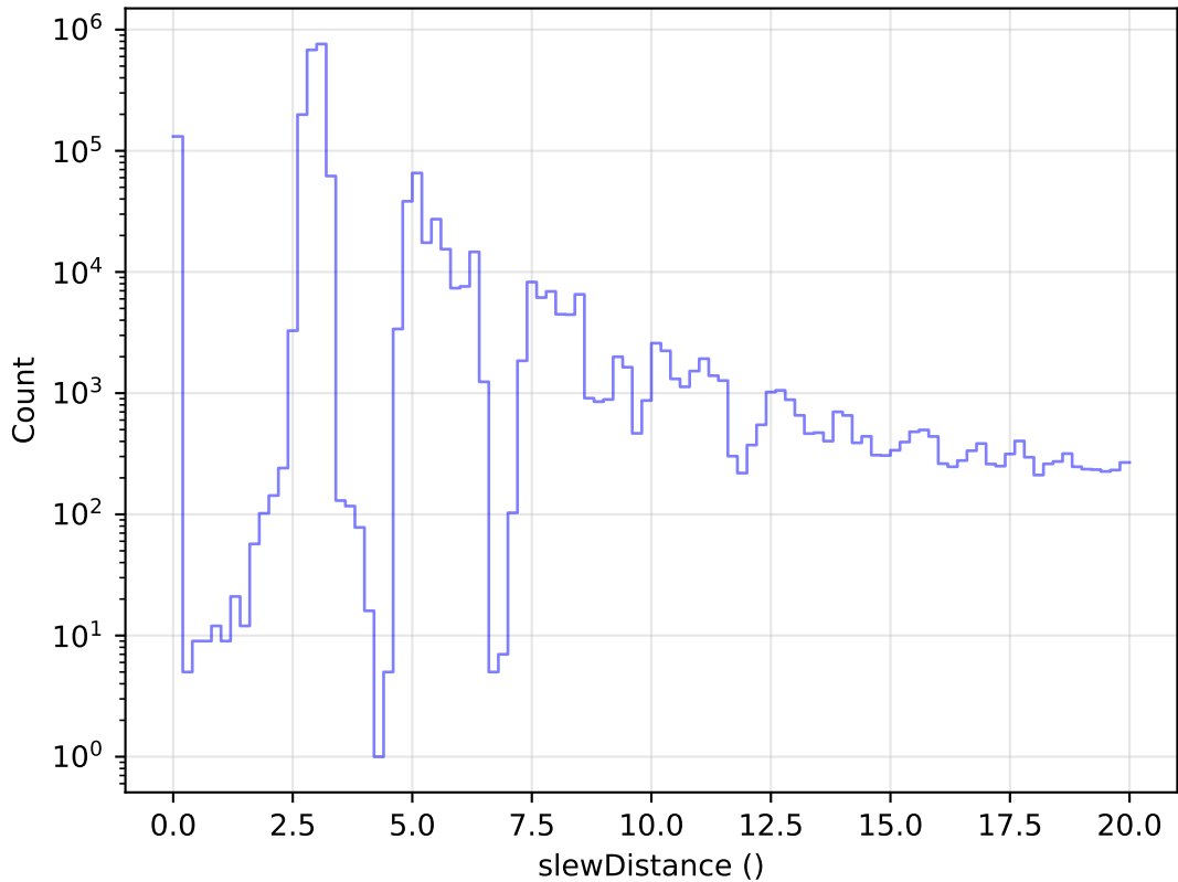
too_elab_2yr_r128_d3_ugrizy_v3.4_10yrs All visits: Zoom Slew Distance Histogram
