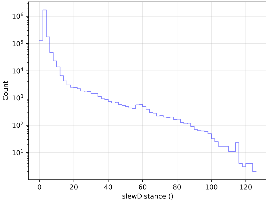
too_elab_2yr_r128_d3_ugrizy_v3.4_10yrs All visits: Slew Distance Histogram
