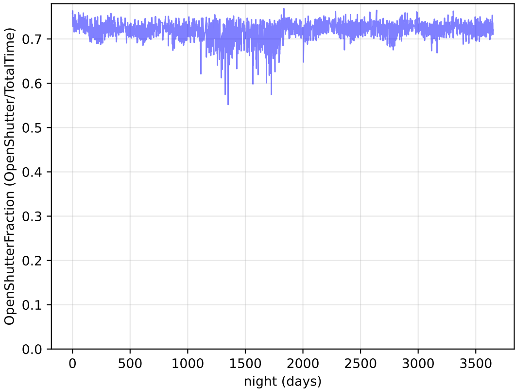
too_elab_2yr_r128_d3_ugrizy_v3.4_10yrs : OpenShutterFraction
