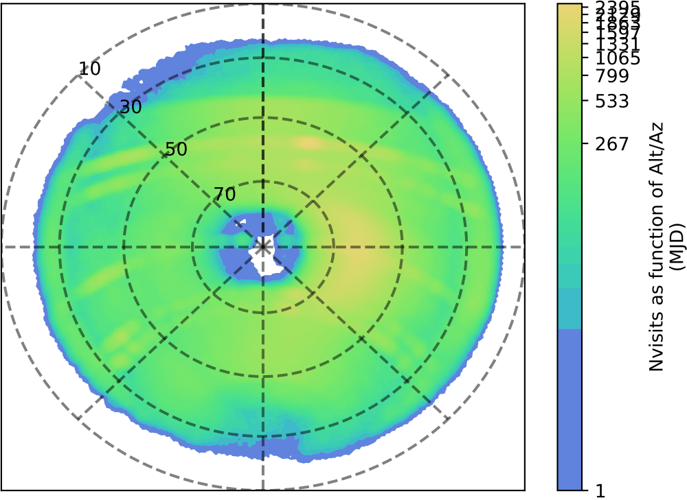
too_elab_2yr_r128_d3_ugrizy_v3.4_10yrs z: Nvisits as function of Alt/Az
