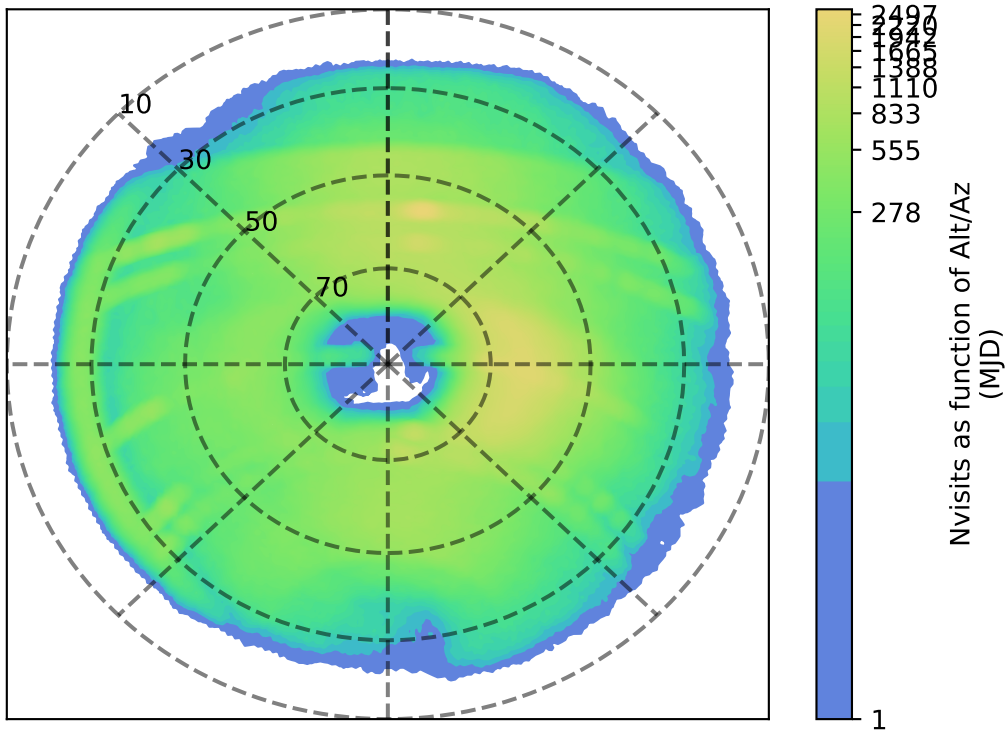
too_elab_2yr_r128_d3_ugrizy_v3.4_10yrs r: Nvisits as function of Alt/Az
