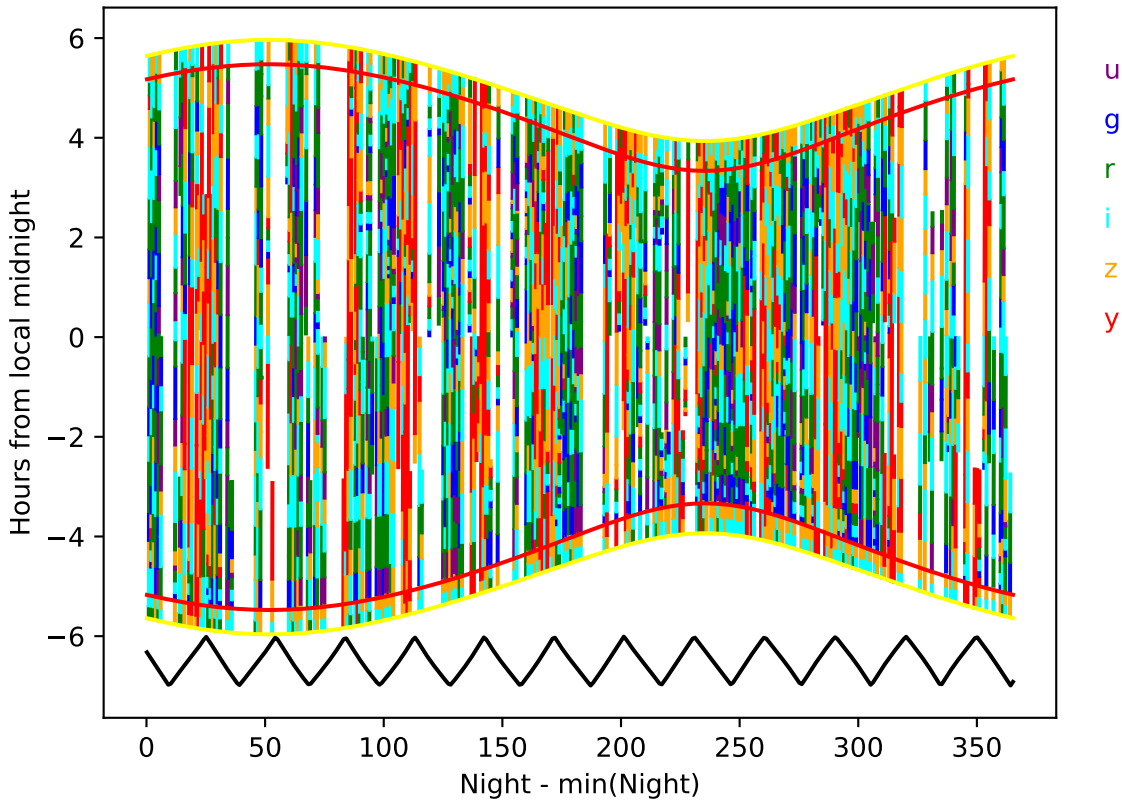
too_elab_2yr_r128_d3_ugrizy_v3.4_10yrs year 7-8: Hourglass
