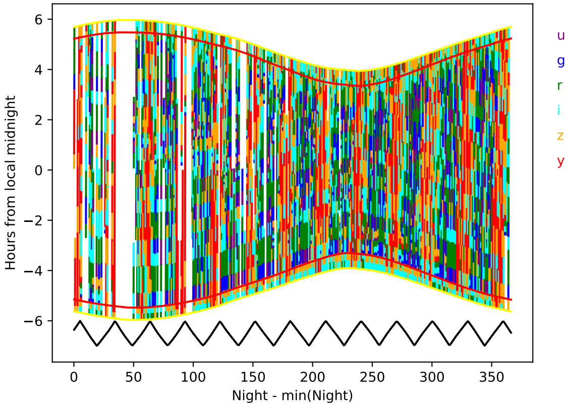
too_elab_2yr_r128_d3_ugrizy_v3.4_10yrs year 6-7: Hourglass
