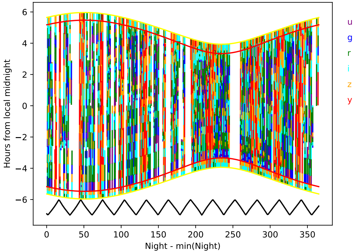
too_elab_2yr_r128_d3_ugrizy_v3.4_10yrs year 5-6: Hourglass
