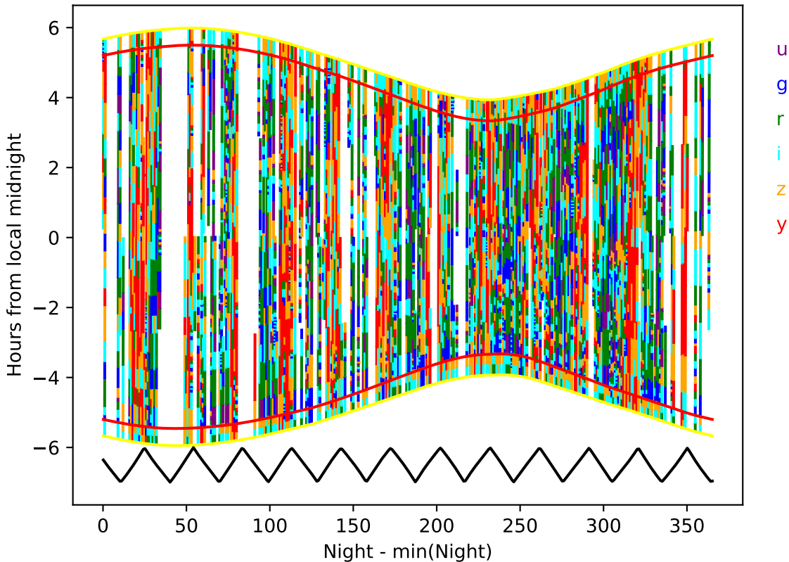
too_elab_2yr_r128_d3_ugrizy_v3.4_10yrs year 4-5: Hourglass
