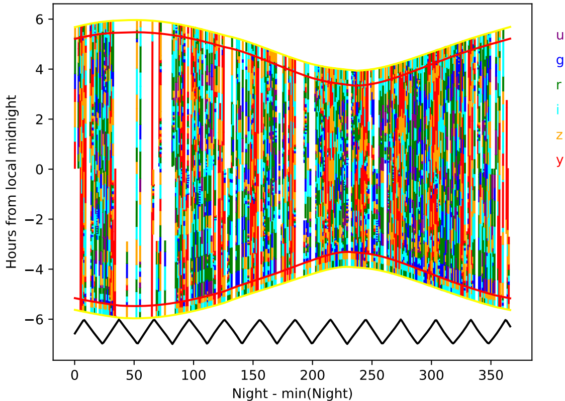
too_elab_2yr_r128_d3_ugrizy_v3.4_10yrs year 3-4: Hourglass
