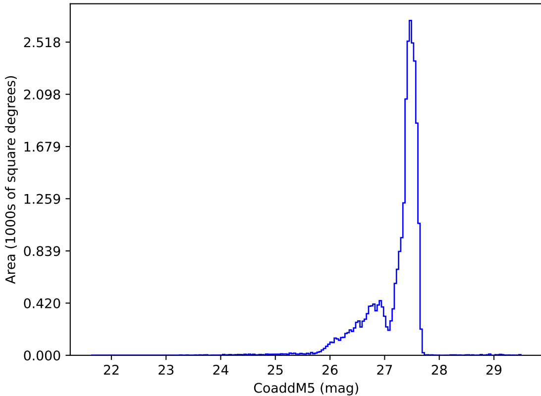
too_elab_2yr_r128_d3_ugrizy_v3.4_10yrs : CoaddM5
