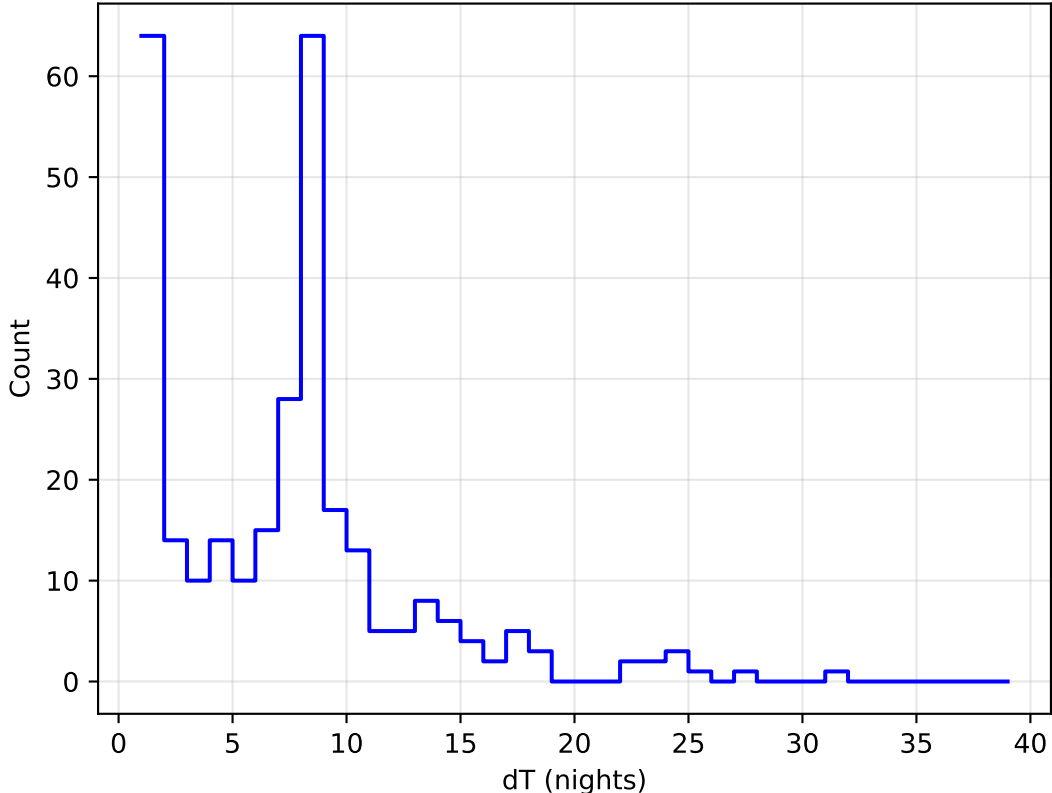
too_elab_2yr_r128_d3_ugrizy_v3.4_10yrs all bands: DD:XMM_LSS Delta Nights Histogram
