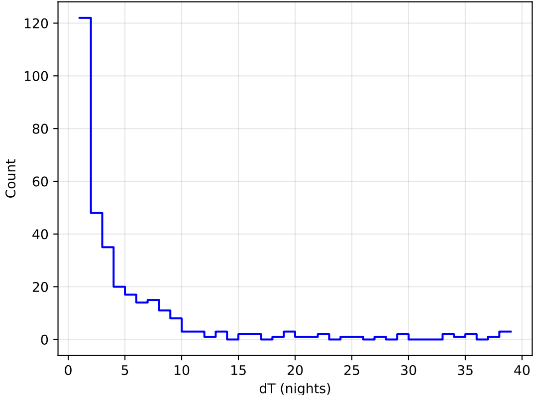
too_elab_2yr_r128_d3_ugrizy_v3.4_10yrs all bands: DD:WFD Delta Nights Histogram
