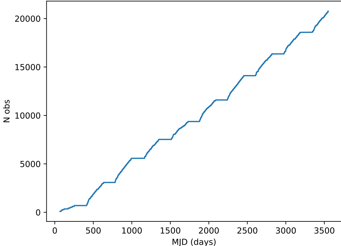
too_elab_2yr_r128_d3_ugrizy_v3.4_10yrs all bands: DD:ELAISS1 Cumulative NVisits
