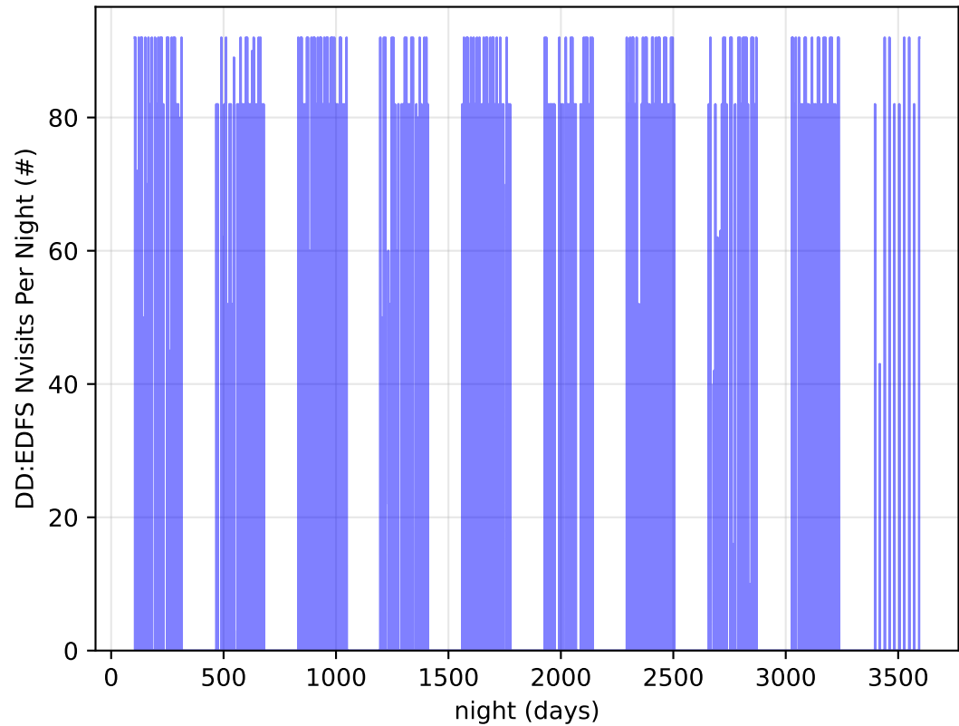
too_elab_2yr_r128_d3_ugrizy_v3.4_10yrs all bands: DD:EDFS Nvisits Per Night
