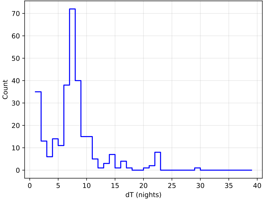
too_elab_2yr_r128_d3_ugrizy_v3.4_10yrs all bands: DD:EDFS Delta Nights Histogram
