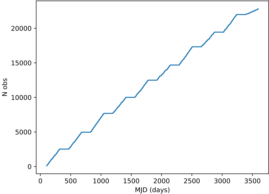
too_elab_2yr_r128_d3_ugrizy_v3.4_10yrs all bands: DD:EDFS Cumulative NVisits
