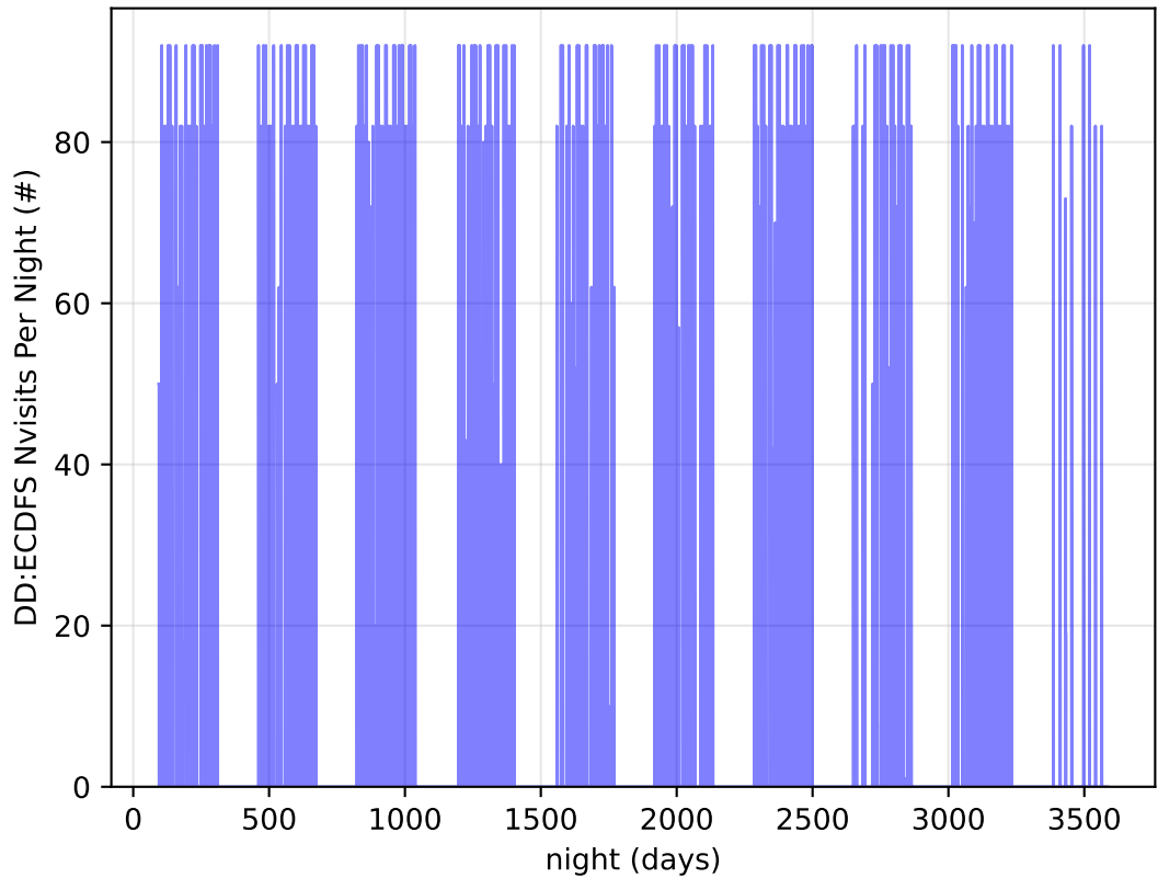
too_elab_2yr_r128_d3_ugrizy_v3.4_10yrs all bands: DD:ECDFS Nvisits Per Night
