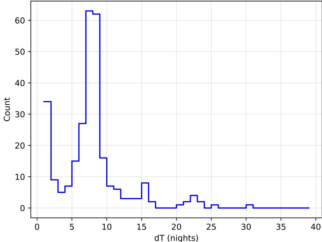
too_elab_2yr_r128_d3_ugrizy_v3.4_10yrs all bands: DD:ECDFS Delta Nights Histogram
