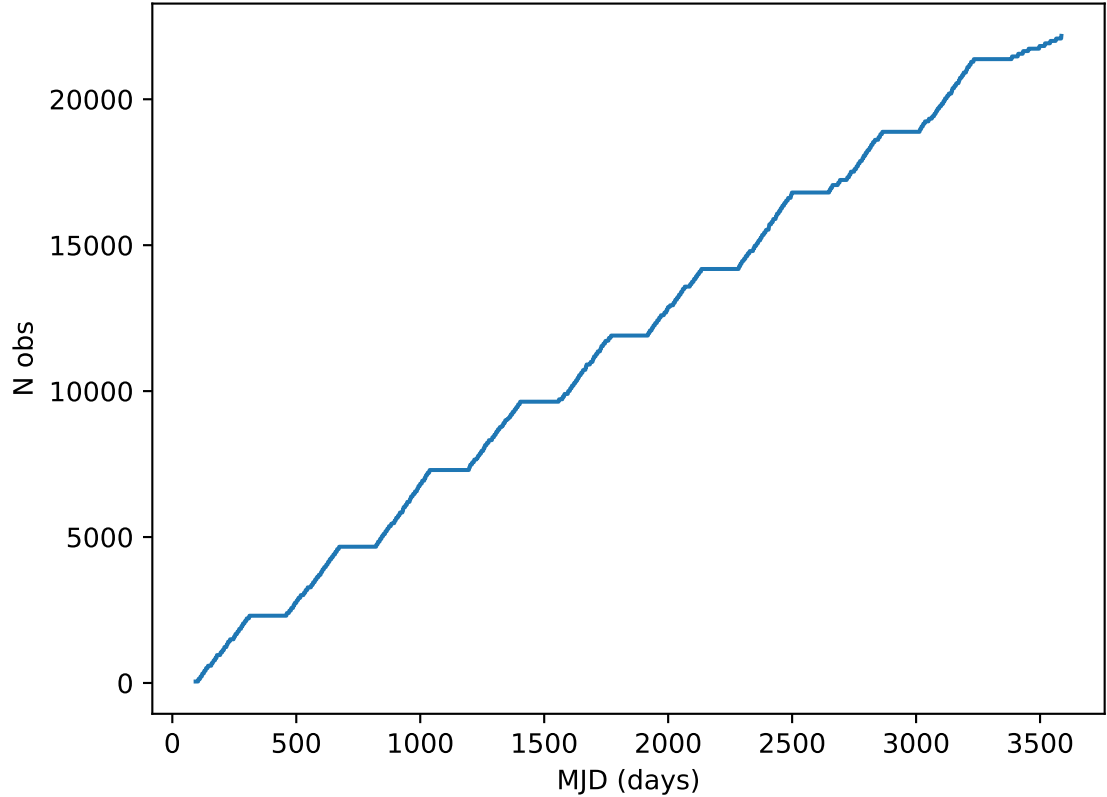
too_elab_2yr_r128_d3_ugrizy_v3.4_10yrs all bands: DD:ECDFS Cumulative NVisits
