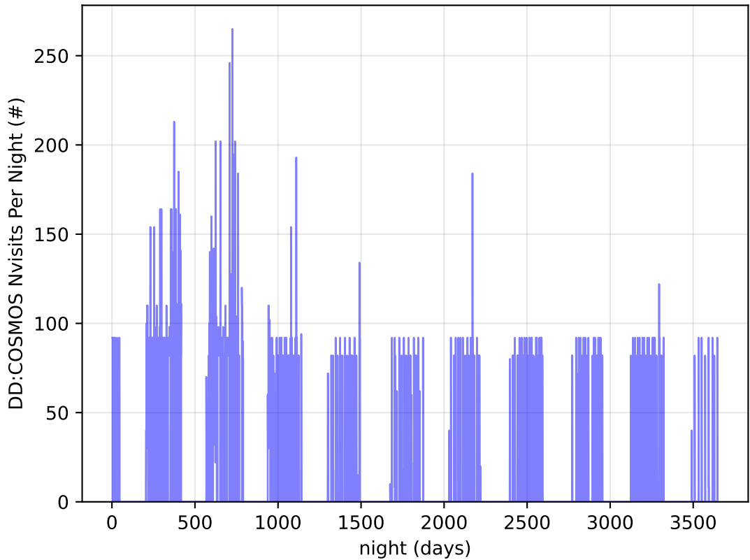
too_elab_2yr_r128_d3_ugrizy_v3.4_10yrs all bands: DD:COSMOS Nvisits Per Night
