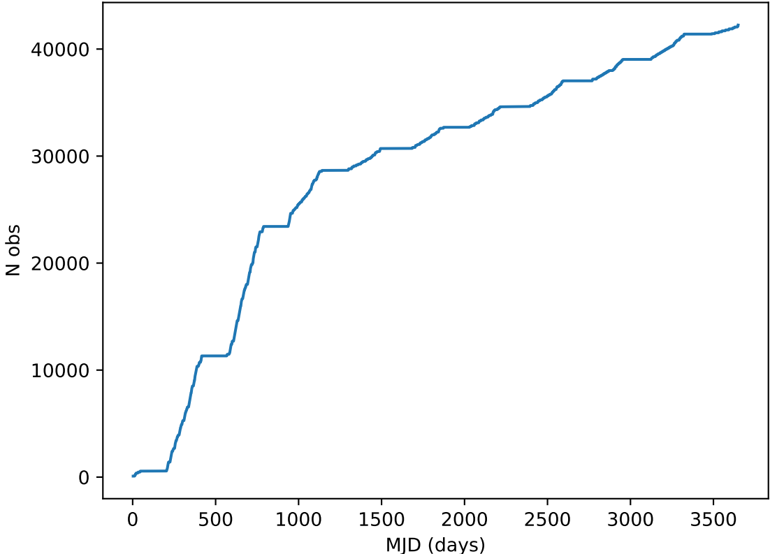
too_elab_2yr_r128_d3_ugrizy_v3.4_10yrs all bands: DD: COSMOS Cumulative NVisits
