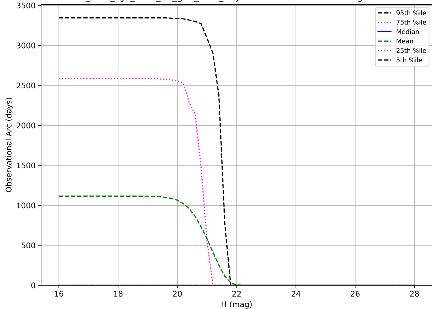
too_elab_2yr_r128_d3_griz_v3.4_10yrs: Observational Arc Length Vatra
