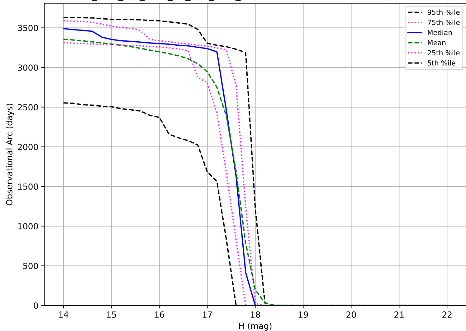
too_elab_2yr_r128_d3_griz_v3.4_10yrs: Observational Arc Length Trojan
