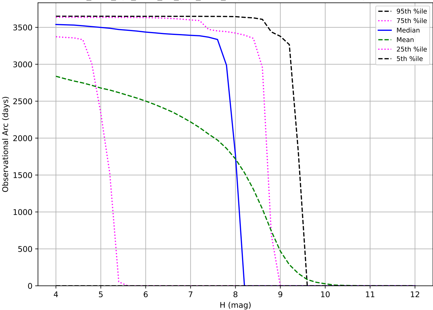
too_elab_2yr_r128_d3_griz_v3.4_10yrs: Observational Arc Length TNO
