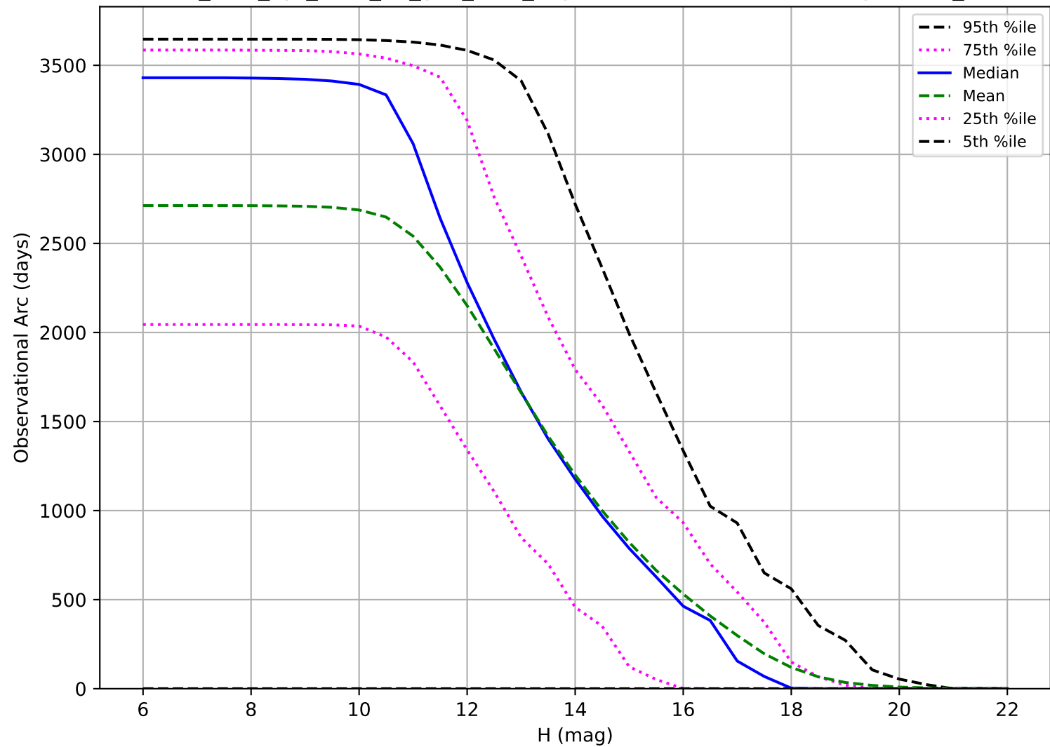
too_elab_2yr_r128_d3_griz_v3.4_10yrs: Observational Arc Length OCC_r5
