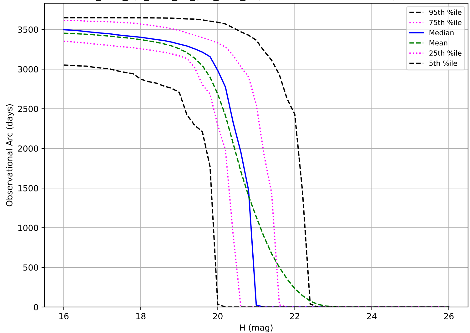
too_elab_2yr_r128_d3_griz_v3.4_10yrs: Observational Arc Length MBA
