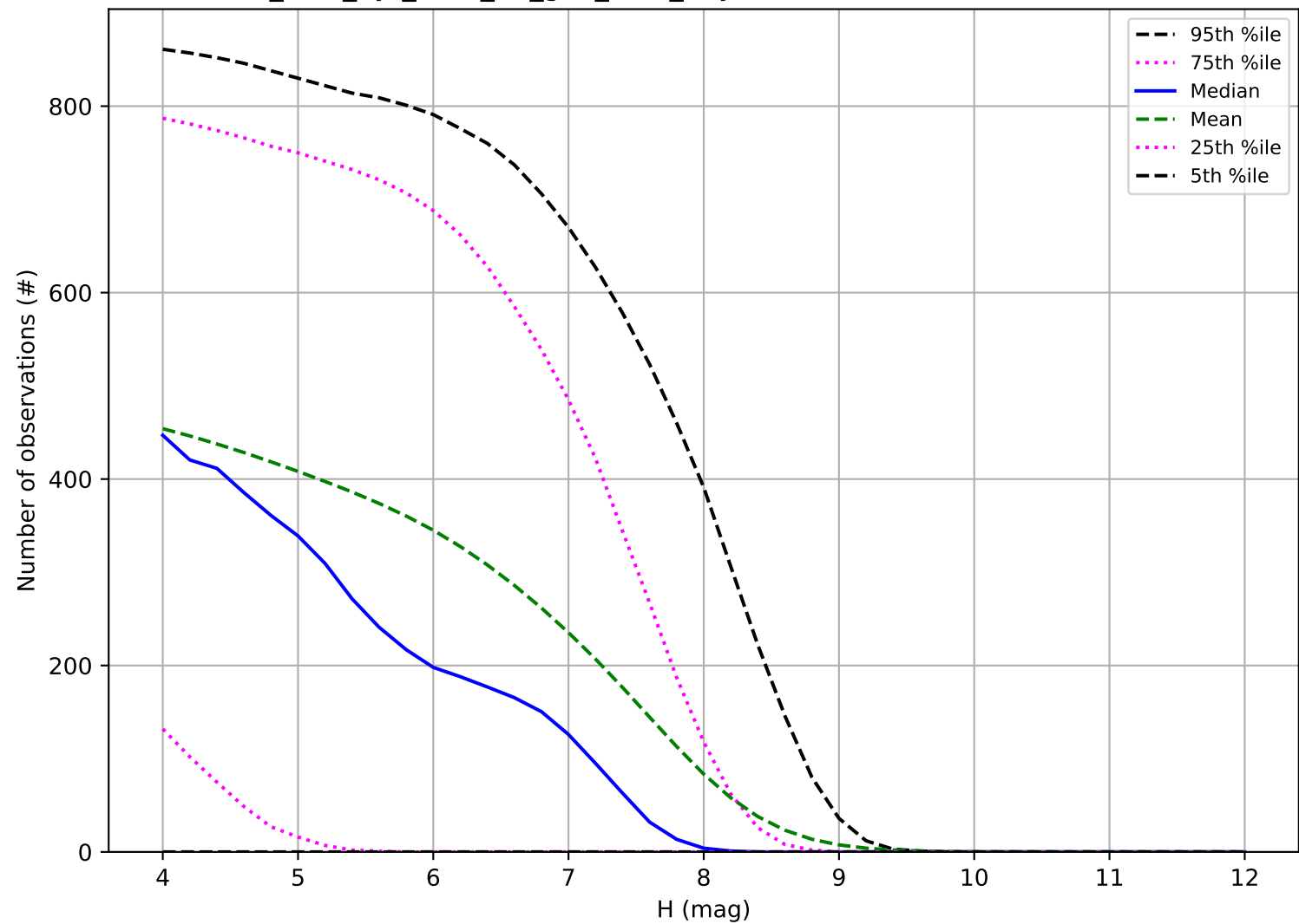
too_elab_2yr_r128_d3_griz_v3.4_10yrs: Number of observations TNO
