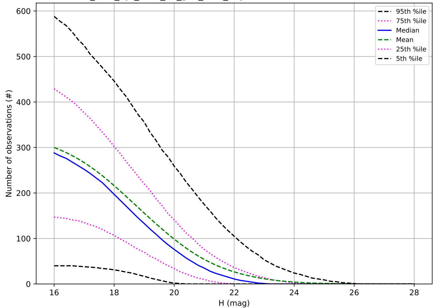
too_elab_2yr_r128_d3_griz_v3.4_10yrs: Number of observations PHA
