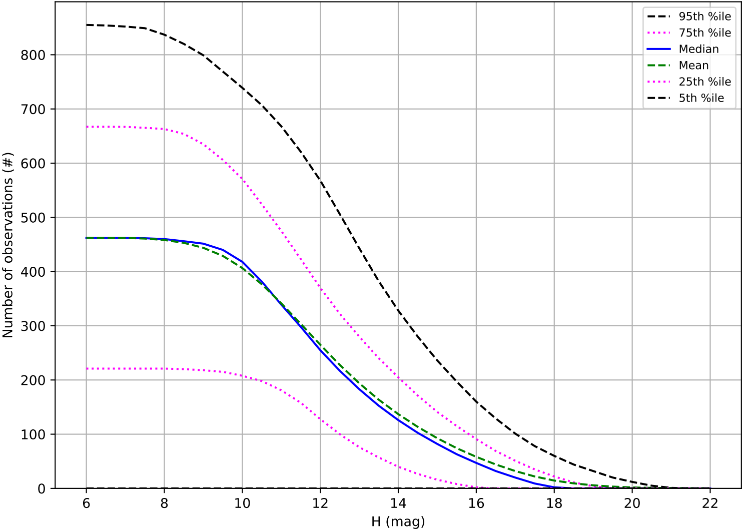
too_elab_2yr_r128_d3_griz_v3.4_10yrs: Number of observations OCC_r5
