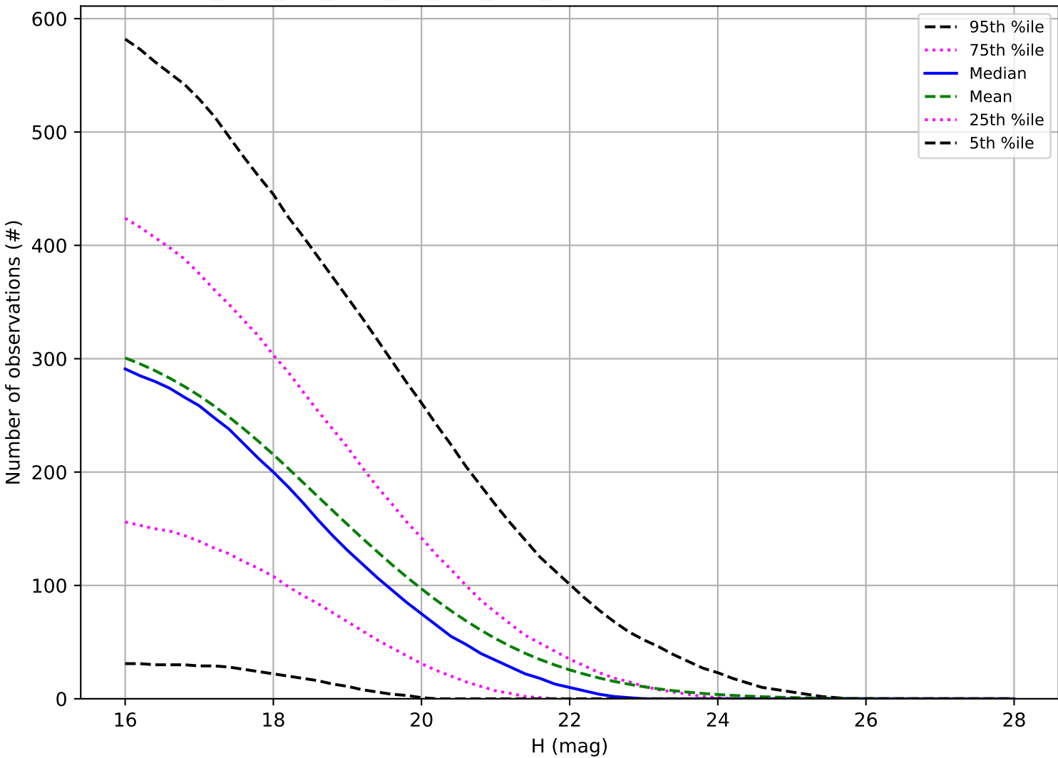
too_elab_2yr_r128_d3_griz_v3.4_10yrs: Number of observations NEO
