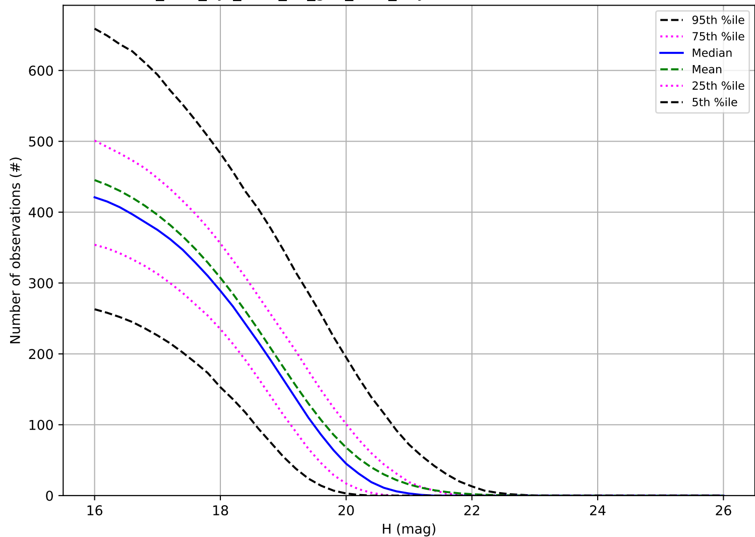
too_elab_2yr_r128_d3_griz_v3.4_10yrs: Number of observations MBA
