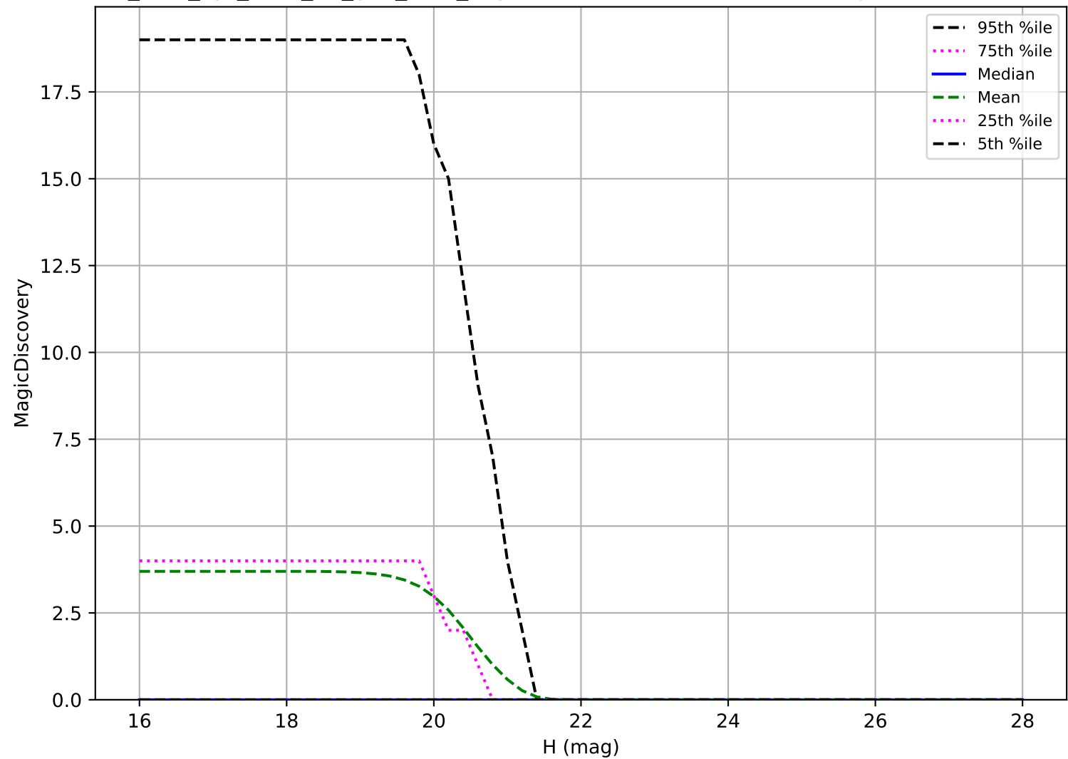
too_elab_2yr_r128_d3_griz_v3.4_10yrs: Vatira 6 detections in 60 nights detection loss
