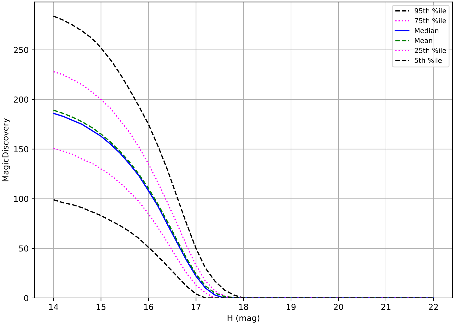
too_elab_2yr_r128_d3_griz_v3.4_10yrs: Trojan 6 detections in 60 nights detection loss
