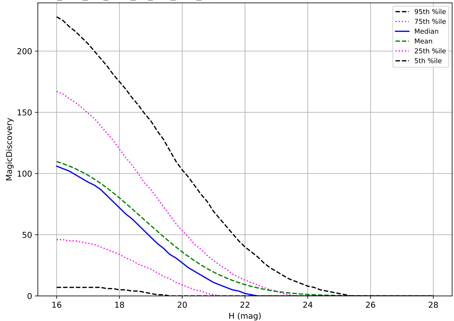
too_elab_2yr_r128_d3_griz_v3.4_10yrs: PHA 6 detections in 60 nights detection loss
