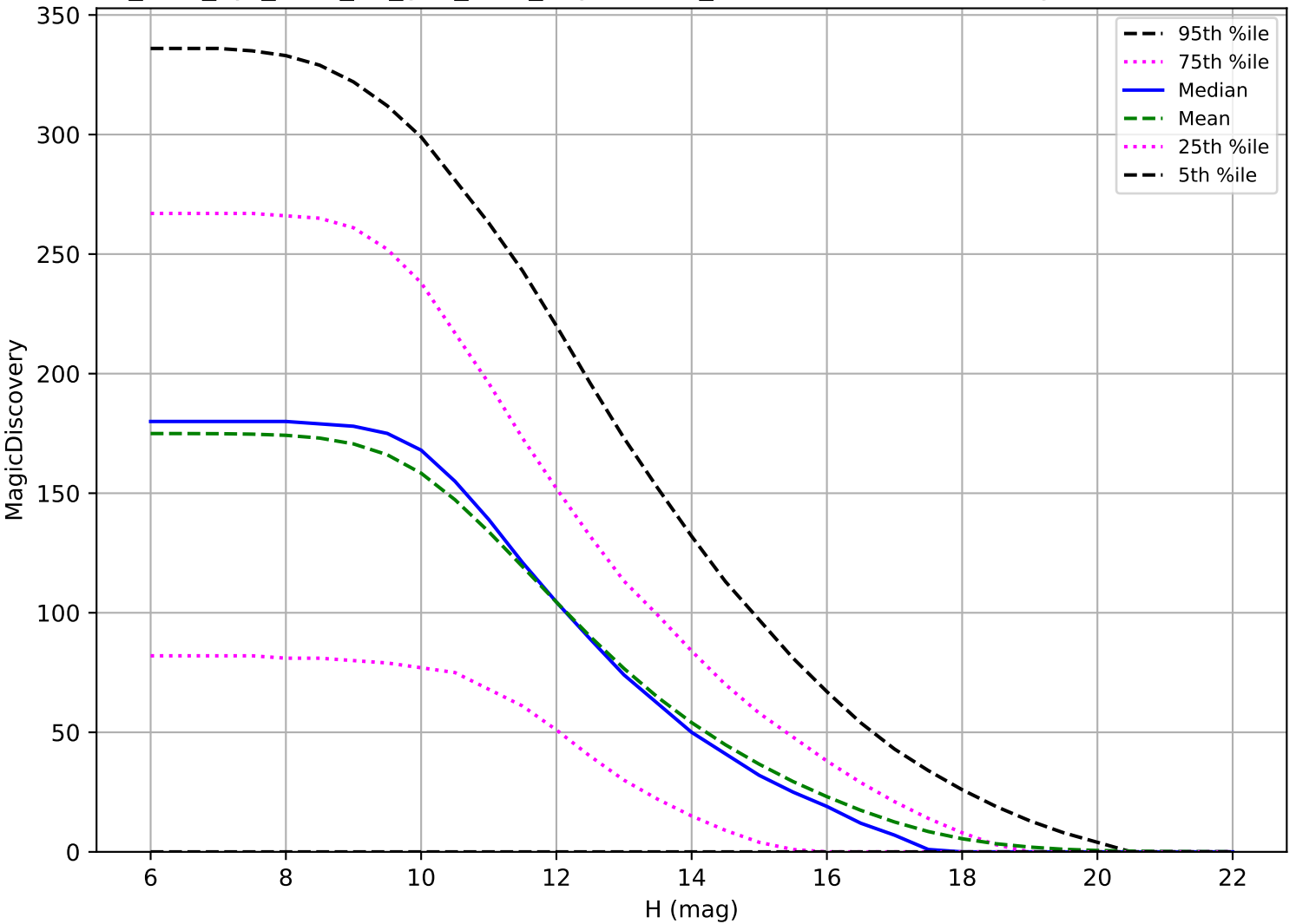
too_elab_2yr_r128_d3_griz_v3.4_10yrs: OCC_r5 6 detections in 60 nights detection loss
