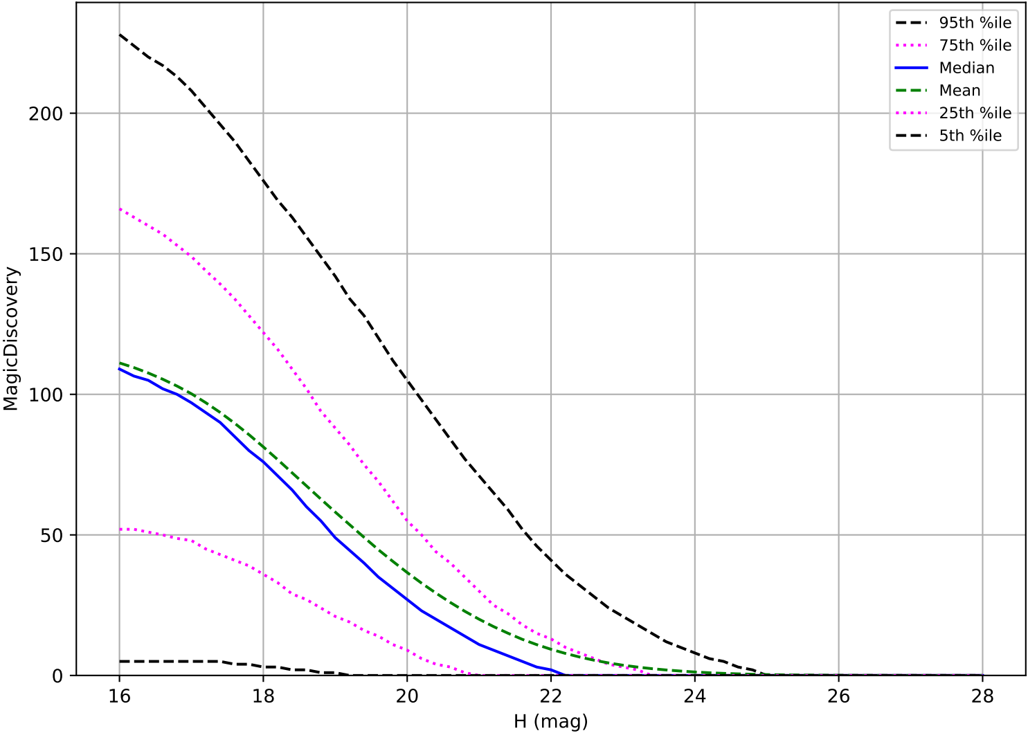
too_elab_2yr_r128_d3_griz_v3.4_10yrs: NEO 6 detections in 60 nights detection loss
