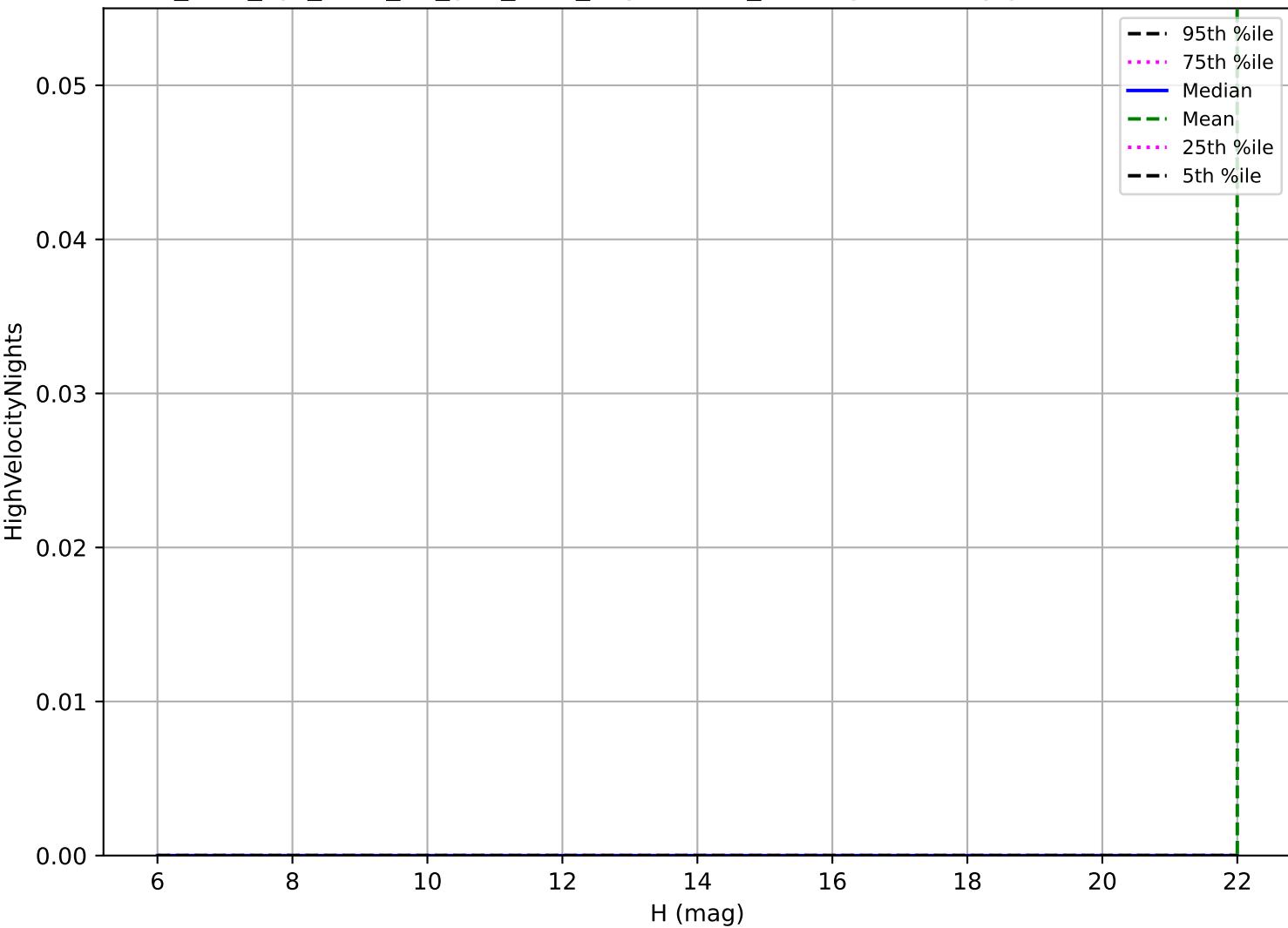
too_elab_2yr_r128_d3_griz_v3.4_10yrs: OCC_r20 High velocity pair detection loss
