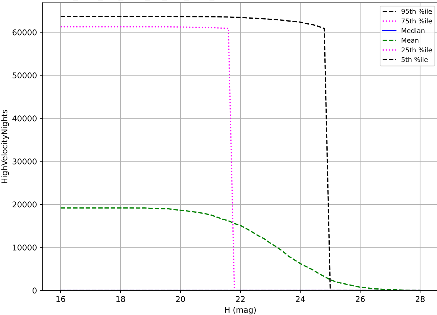
too_elab_2yr_r128_d3_griz_v3.4_10yrs: NEO High velocity pair detection loss
