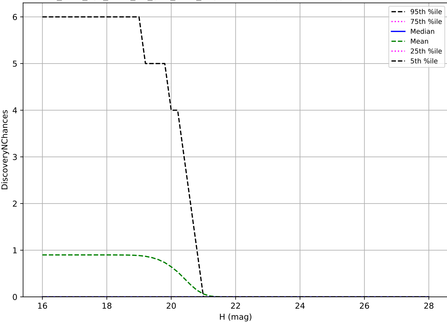
too_elab_2yr_r128_d3_griz_v3.4_10yrs: Vatira 3 pairs in 15 nights detection loss
