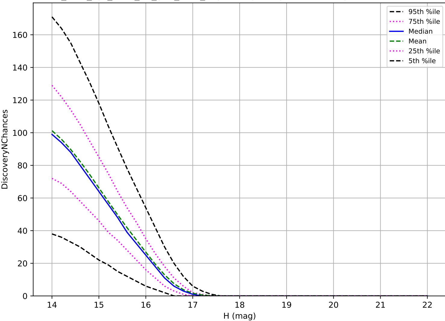
too_elab_2yr_r128_d3_griz_v3.4_10yrs: Trojan 3 pairs in 15 nights detection loss
