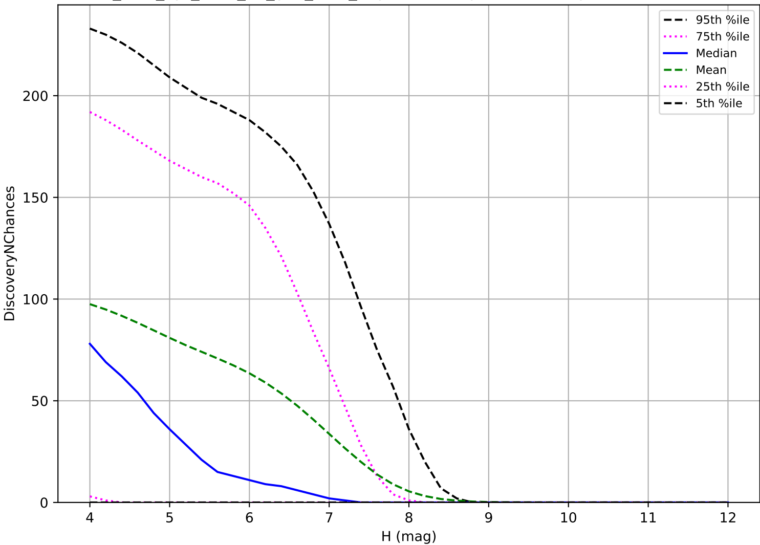
too_elab_2yr_r128_d3_griz_v3.4_10yrs: TNO 3 pairs in 15 nights detection loss
