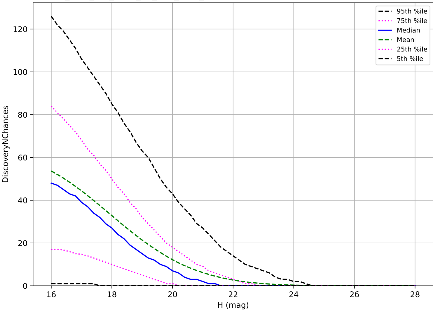
too_elab_2yr_r128_d3_griz_v3.4_10yrs: PHA 3 pairs in 15 nights detection loss
