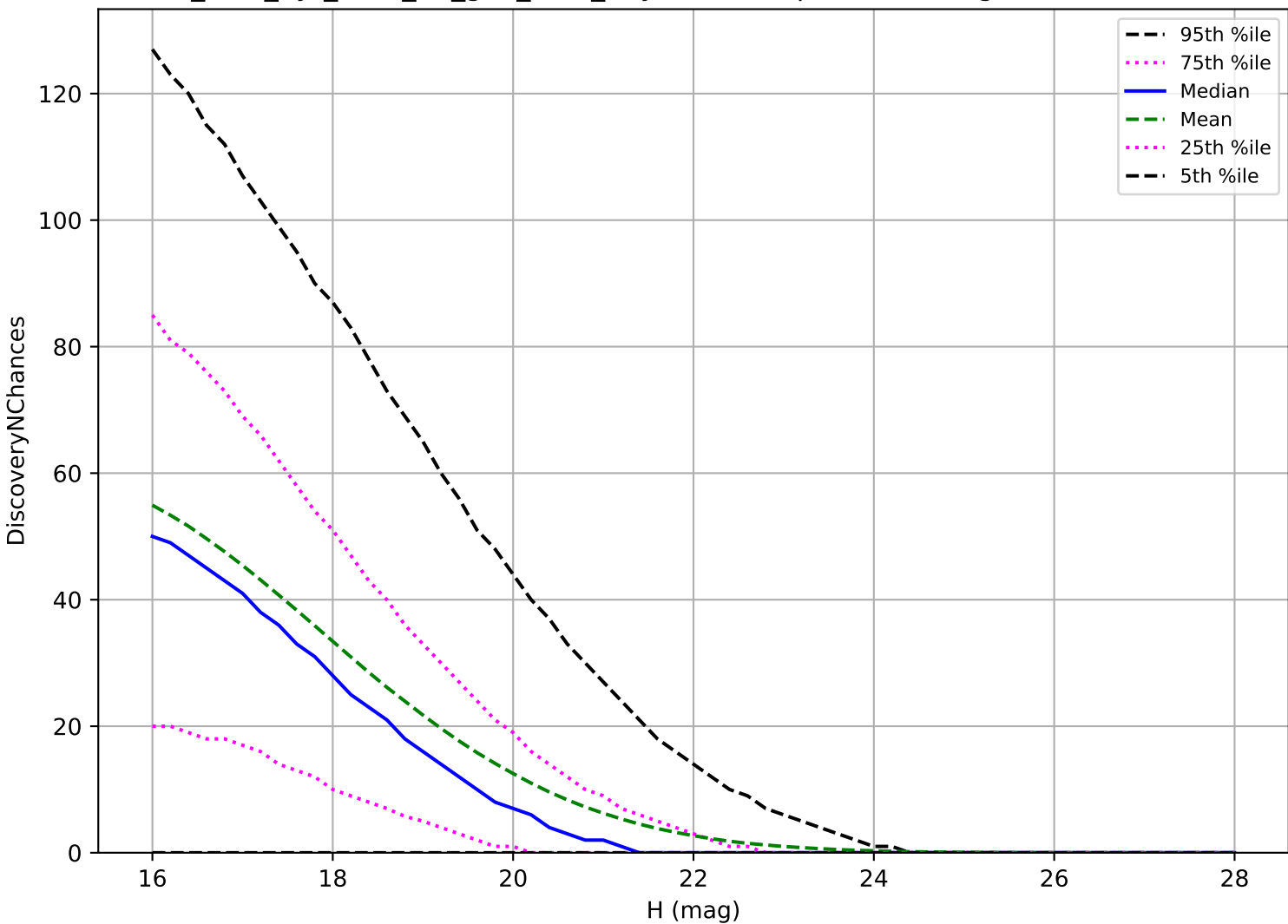
too_elab_2yr_r128_d3_griz_v3.4_10yrs: NEO 3 pairs in 15 nights detection loss
