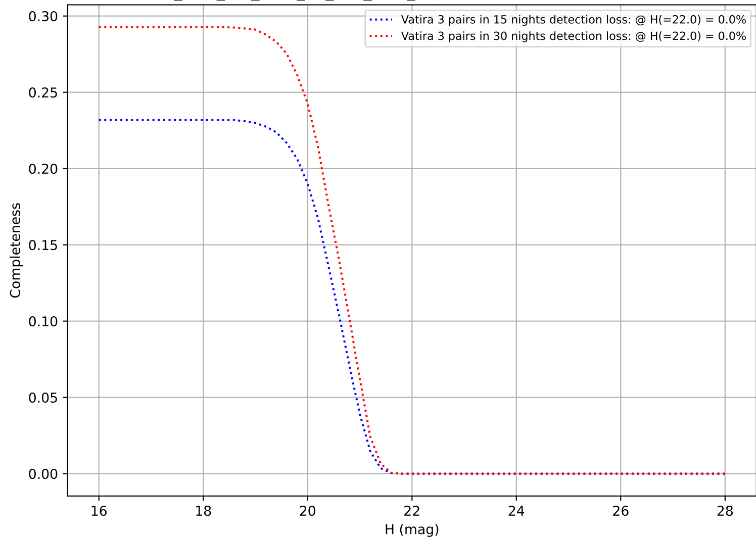
too_elab_2yr_r128_d3_griz_v3.4_10yrs: DifferentialCompleteness
