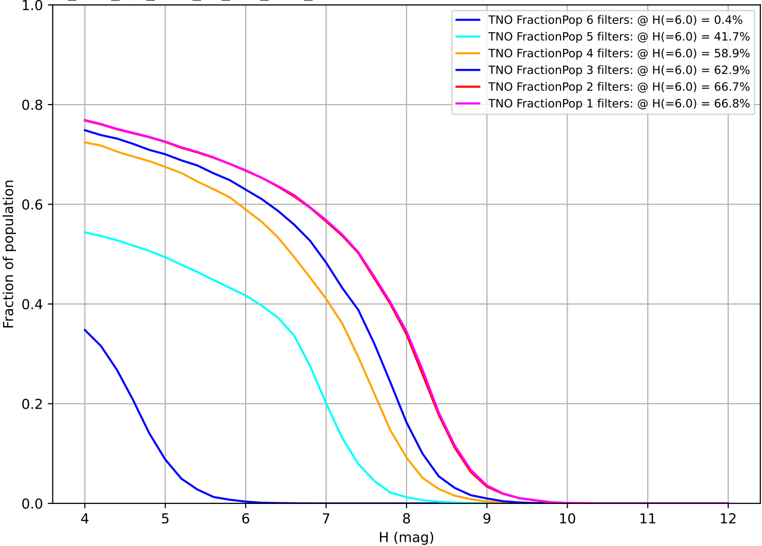
too_elab_2yr_r128_d3_griz_v3.4_10yrs: Fraction of population with colors in X filters TNO
