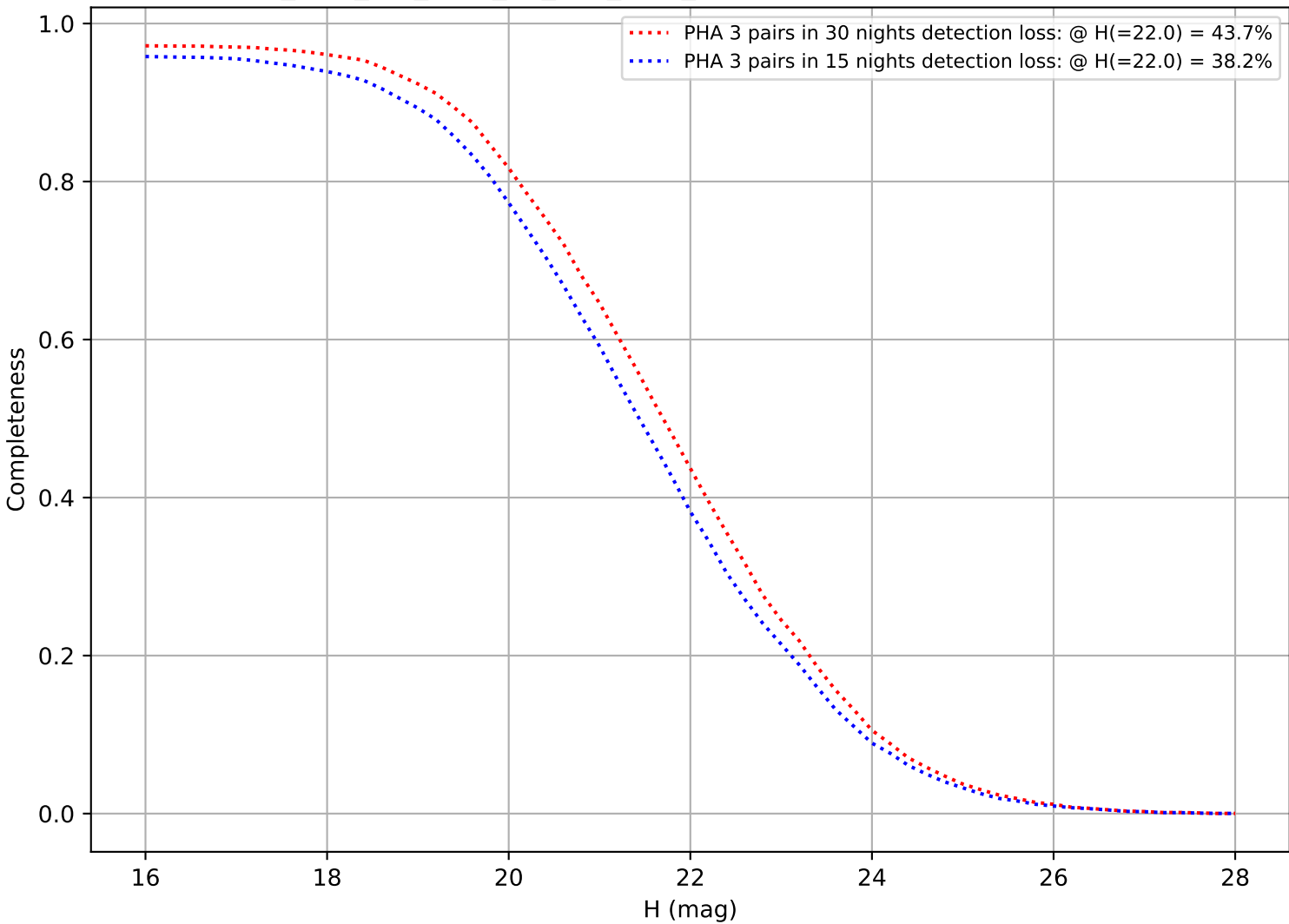
too_elab_2yr_r128_d3_griz_v3.4_10yrs: DifferentialCompleteness
