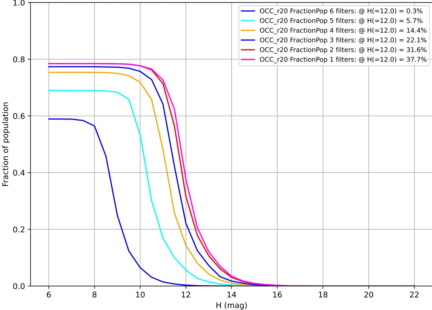
too_elab_2yr_r128_d3_griz_v3.4_10yrs: Fraction of population with colors in X filters OCC_r20
