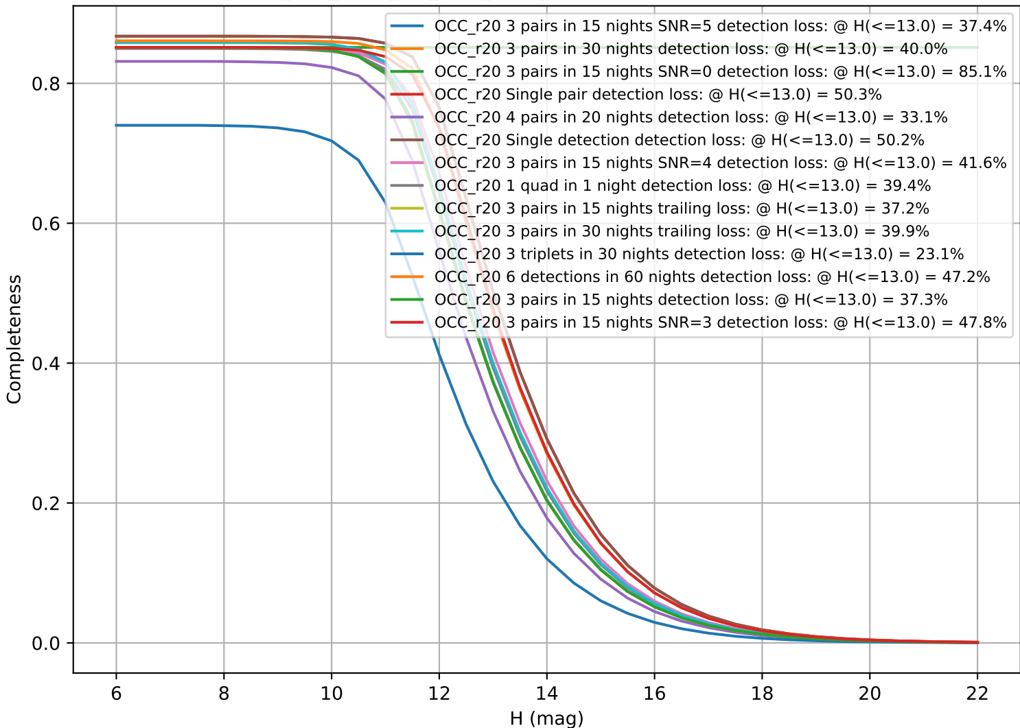
too_elab_2yr_r128_d3_griz_v3.4_10yrs: CumulativeCompleteness
